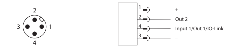
Wiring diagram of primary side
