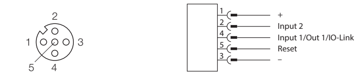
Wiring diagram of secondary side
